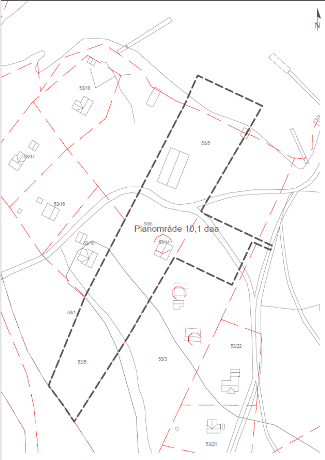
Figur 2 Planomriss
